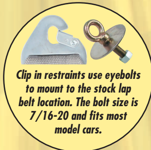
Clip-In
